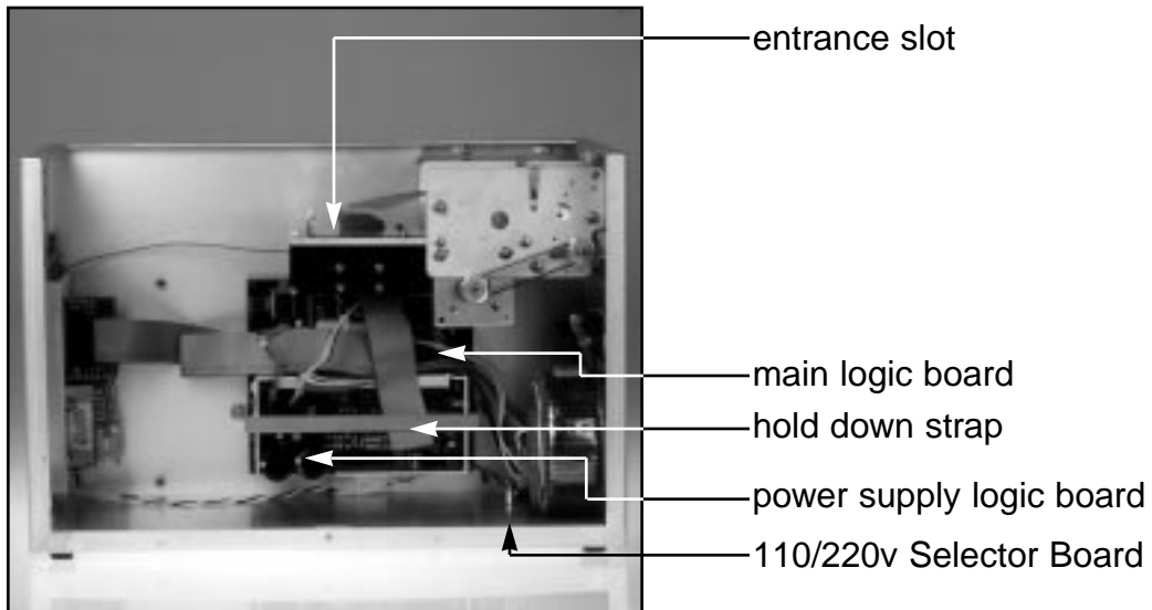
Figure 5 - Micro Plus side view with electronics exposed
