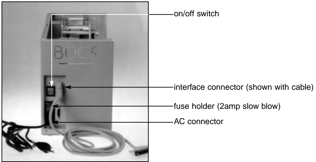
Figure 4 - Micro Plus rear view
