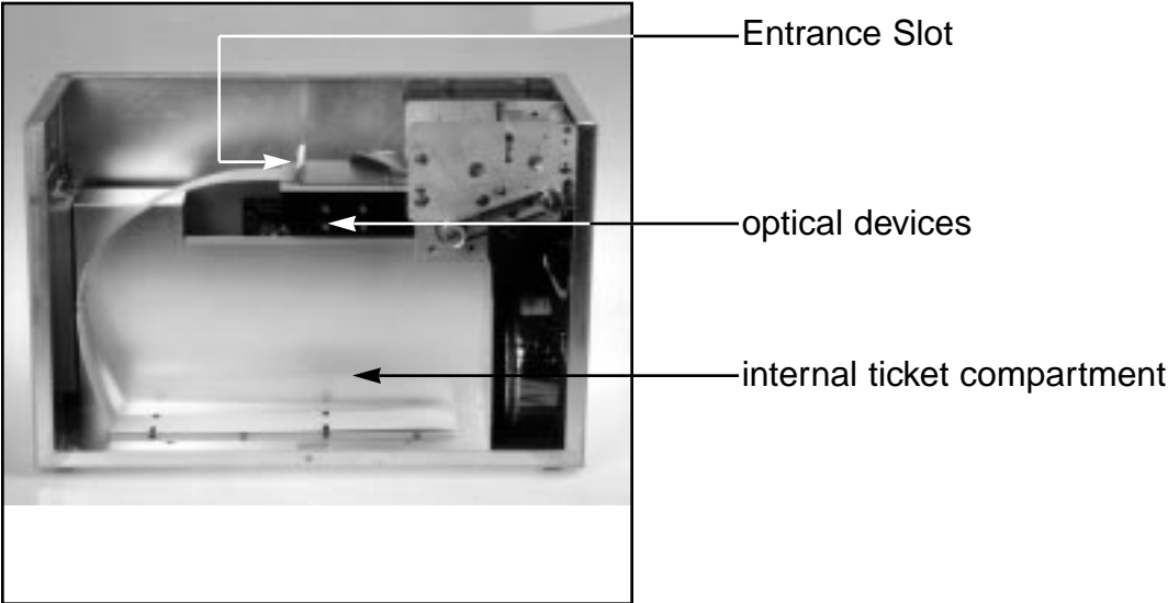
Figure 3 - Micro Plus side view
