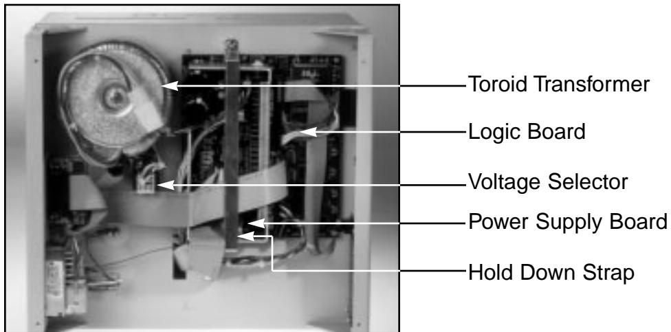
Figure 5 - Dual Mini bottom view (cover removed)
