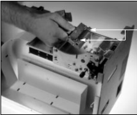
Figure 8B - Print Head removal
