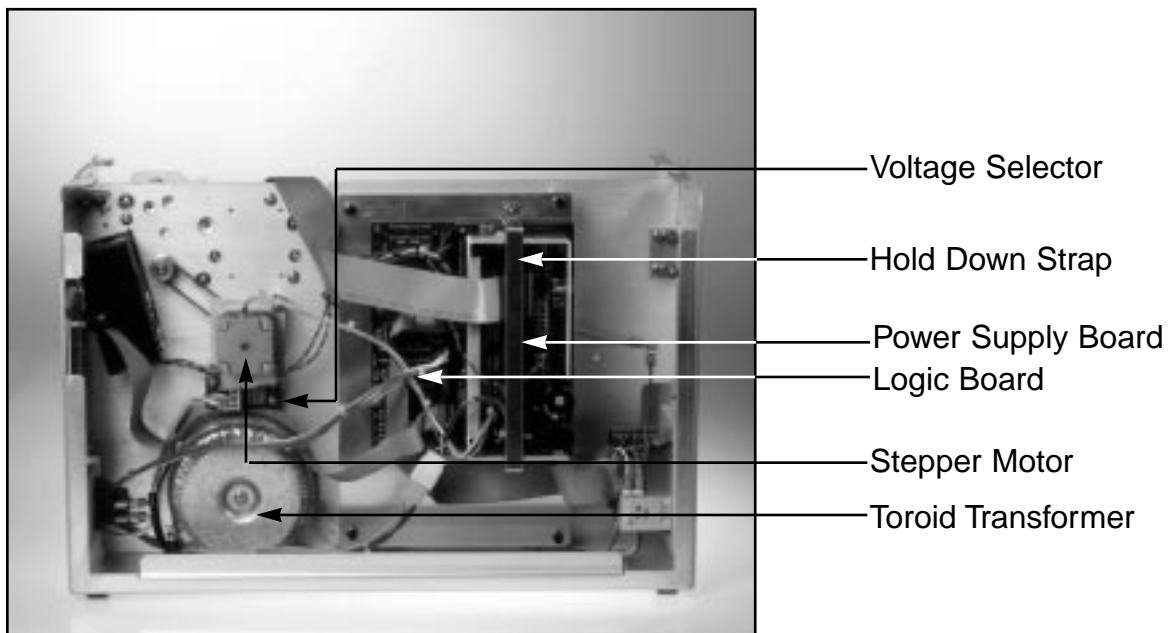
Figure 3b - Mini Plus side view Electronics Cover Removed
