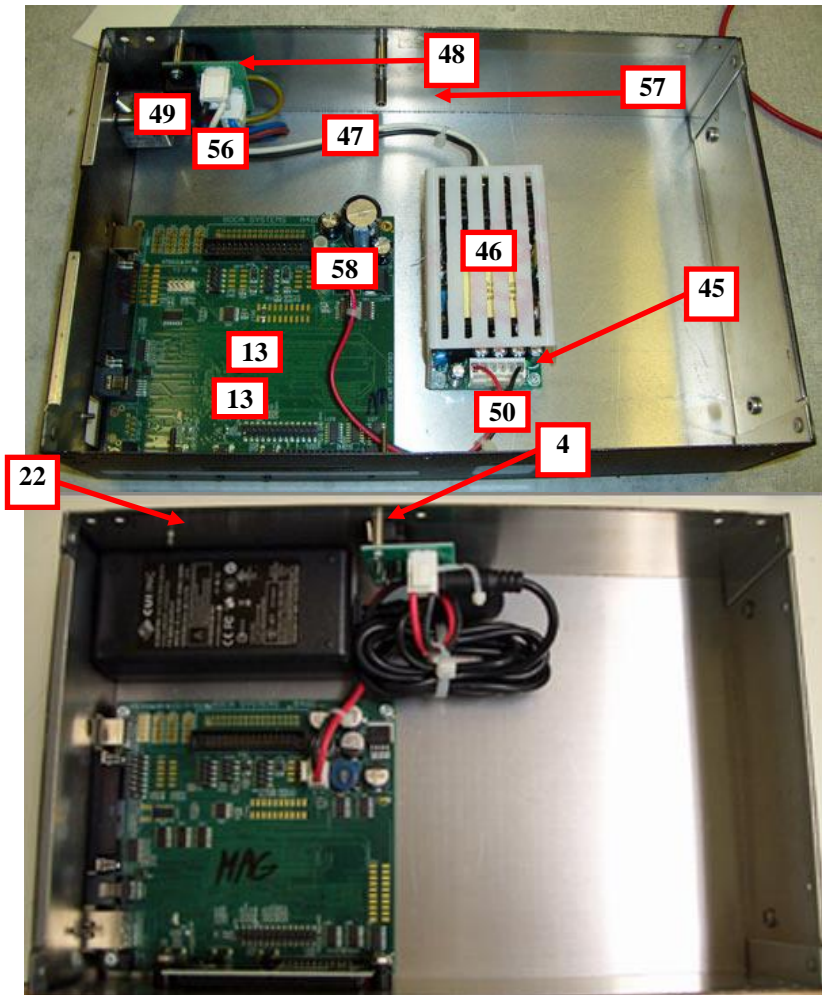
Printers built after June 2016 used the above configuration
